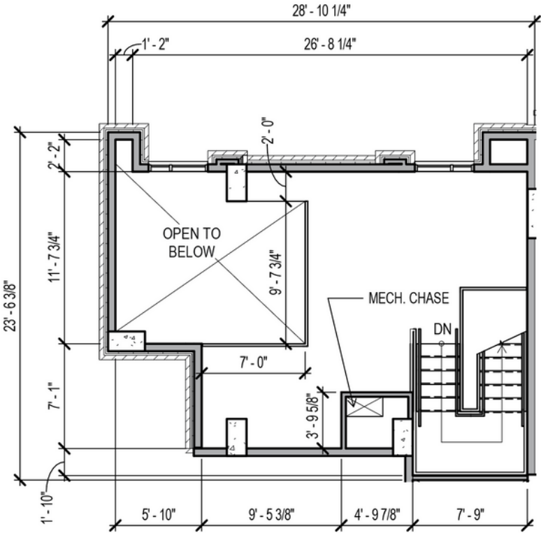
MEZZANINE
