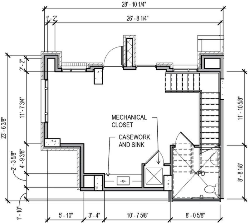
MAIN LEVEL
